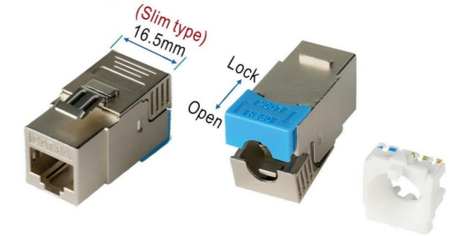
A: Cat.6A STP RJ45 Keystone Jack B: Cat.6 STP RJ45 Keystone Jack Toolless Type
